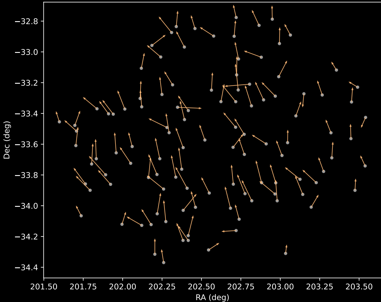
GALAH DR4 Cluster 3 Proper Motion Vectors (n=111)
