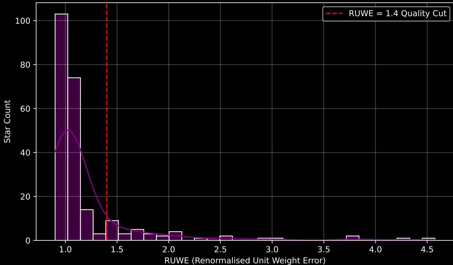
GALAH DR4 Field [3141] RUWE Distribution (n= 230)
