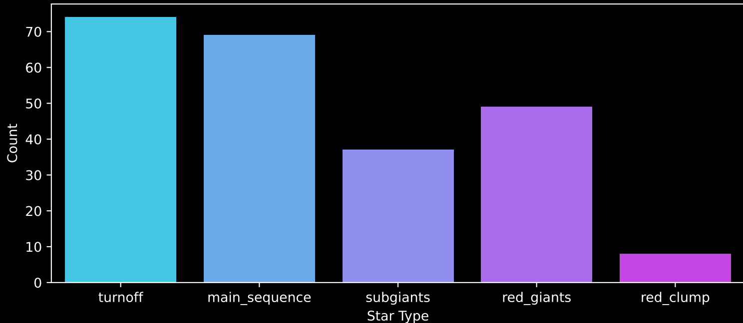
GALAH DR4 Field: [3141] Count plot of Star Type
