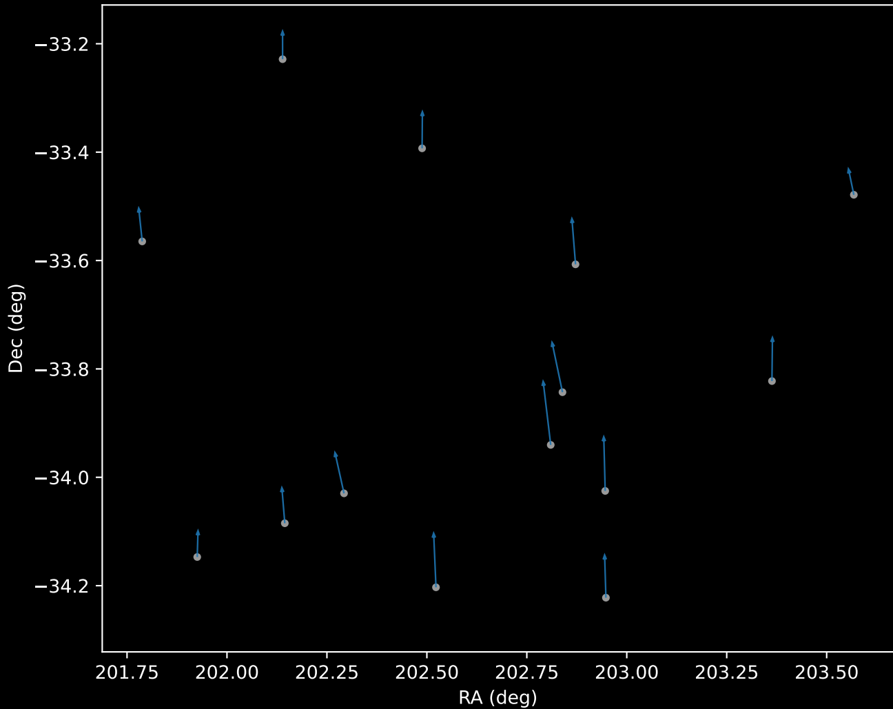
GALAH DR4 Cluster 0 Proper Motion Vectors (n=14)
